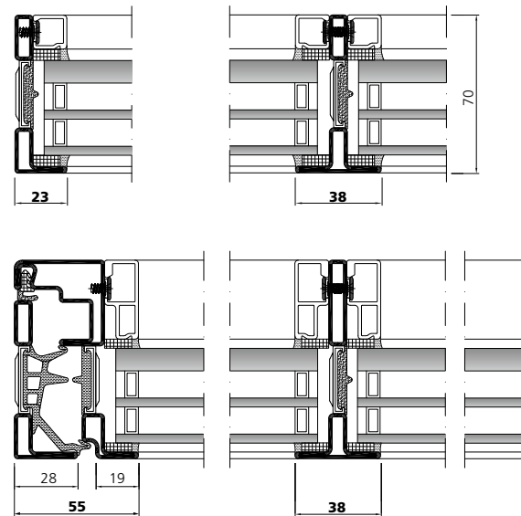
Einbruchhemmung forster unico XS Forster unico XS anti-effraction Forster unico XS burglary-resistance
