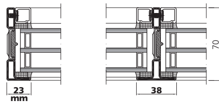
Verglasung forster unico XS Vitrage forster unico XS Glazing forster unico XS
