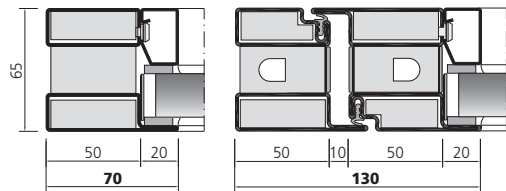
EI60 Tür, Verglasung Porte, Cloison EI60 Door, glazing EI60
