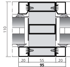
EI120 Verglasung Cloison EI120 Glazing EI120
