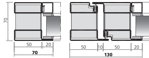
EI90 Tür, Verglasung Porte, Cloison EI90 Door, glazing EI90
