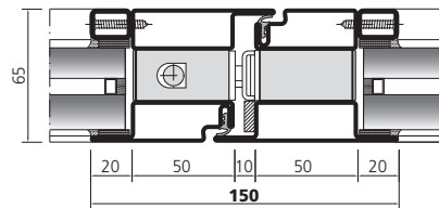
EI30 Einbruchhemmende Tür RC2 Porte EI30 anti-effraction CR2 Door EI30 with burglary-resistance
