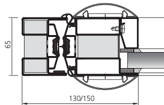
EI30 Fingerschutztür Porte anti-pince doigts EI30 Anti-finger trap door EI30
