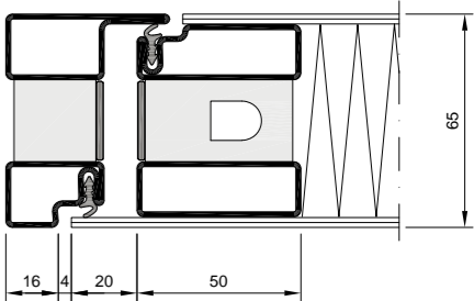
Door leaf Frame combination Flush sheet metal
