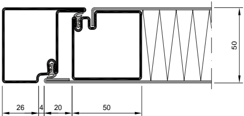
Door leaf Frame combination flush sheet metal
