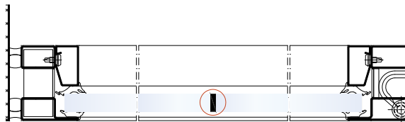
EI30 Verglasung Glas-Glas-Stoss, Fuge 4 mm Cloison EI30 bords à bords, joint 4 mm Glazing EI30 glass-to-glass with 4 mm joint
